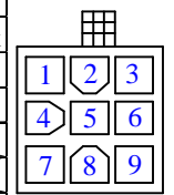
Encoder Connection
