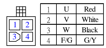
Motor Connection
